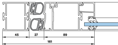
Klemfri bakkant, gummilister
